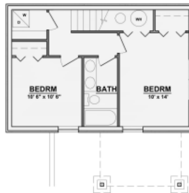
LOWER LEVEL FLOOR PLAN SCALE 1/8" = 1'-0"
